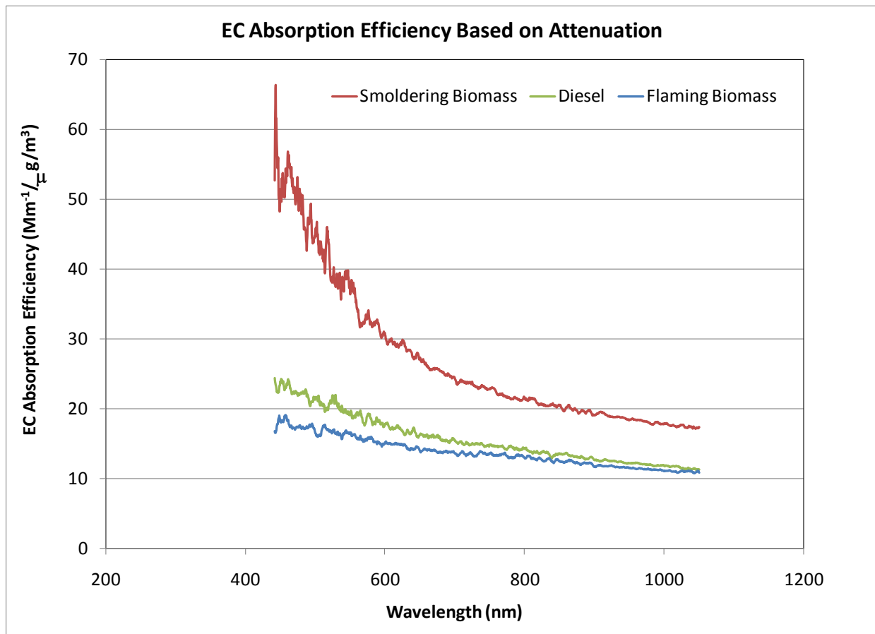
Figure 2. Absorption efficiencies as a function of wavelength for biomass smoldering, biomass flaming, and diesel exhaust. EC was measured by the IMPROVE thermal/optical reflectance method and light transmission was measured with an Oceans Optic spectrophotometer. Biomass burned consisted of moist (smoldering) and dry squaw carpet stems (data from Chen et al. 2010). Diesel exhaust was generated with an Onan Cummins diesel generator operating at 32% of full capacity (Chow et al. 2006). Filter transmittance attenuation is correlated with, but not the same as, particle absorption in the atmosphere owing to scattering within the filter and changes in particle shape after collection on the filter (Chow et al. 2010).
